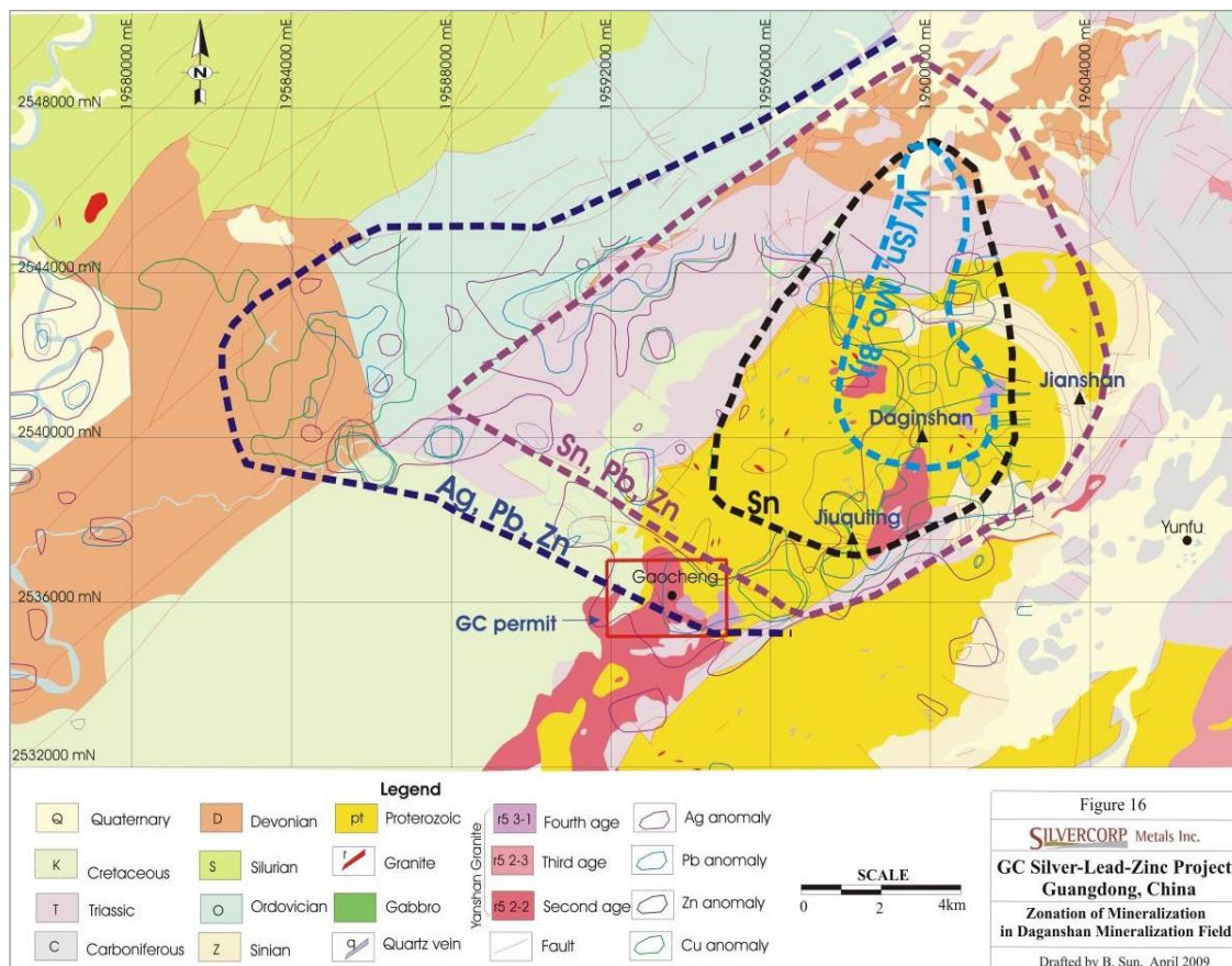
Figure 23.1 Zonation of mineralization in the Dagenshan mineralization field
